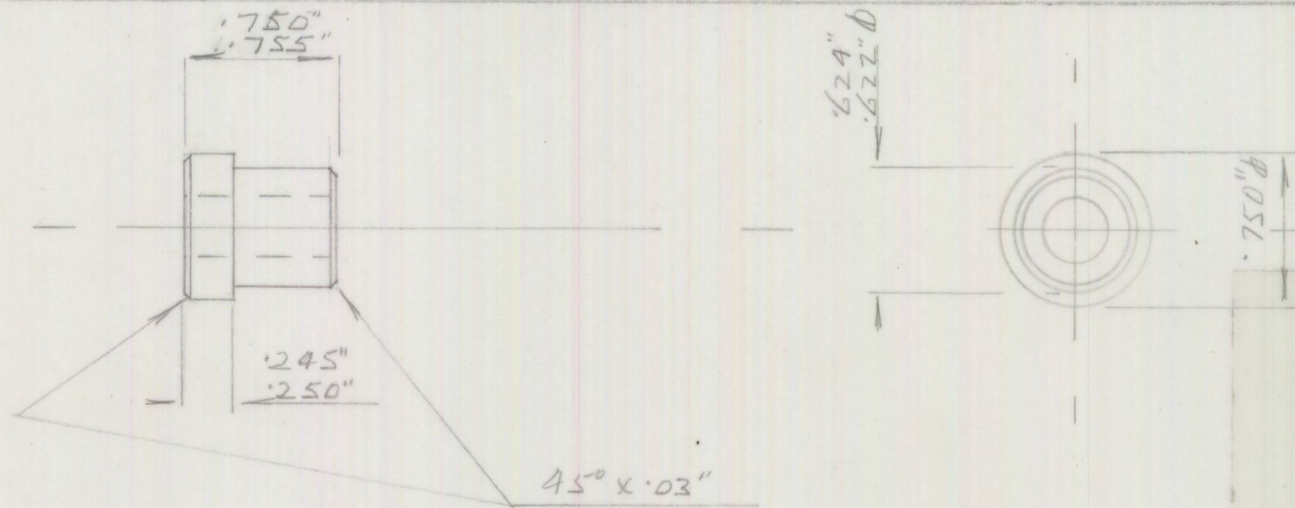
PIVOT BUSH. CLUTCH PEDAL - 2 OFF
