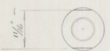
END VIEW OF BUSH SHOWING SPANNER FLATS
