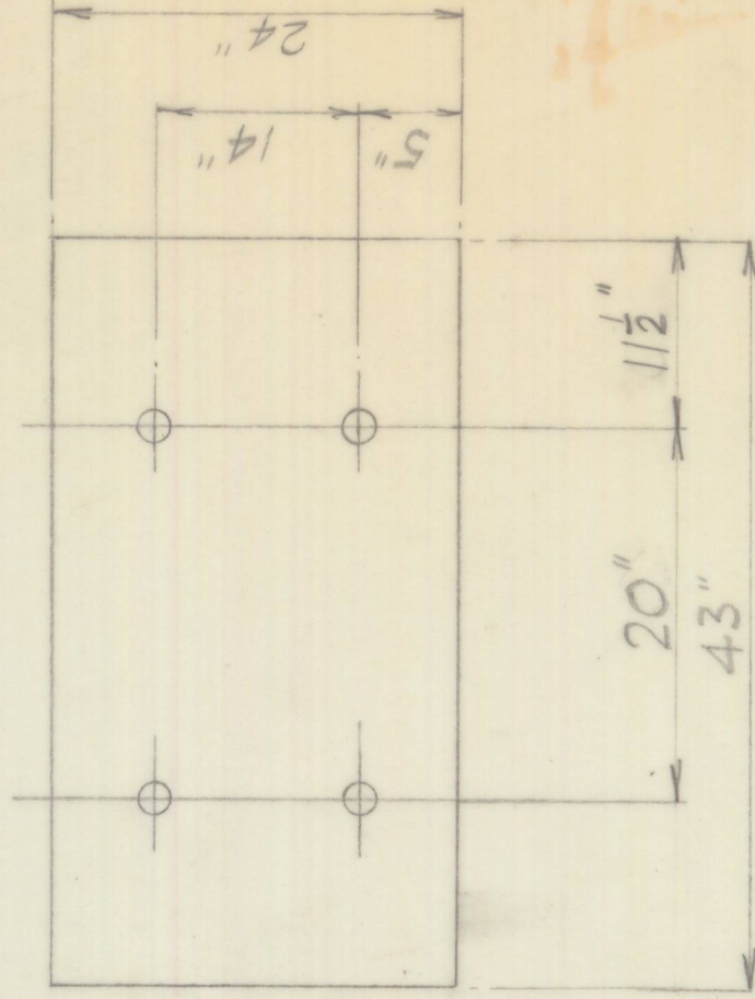
VIEW ON U/SIDE SHOWING POSN OF INSERTS.
