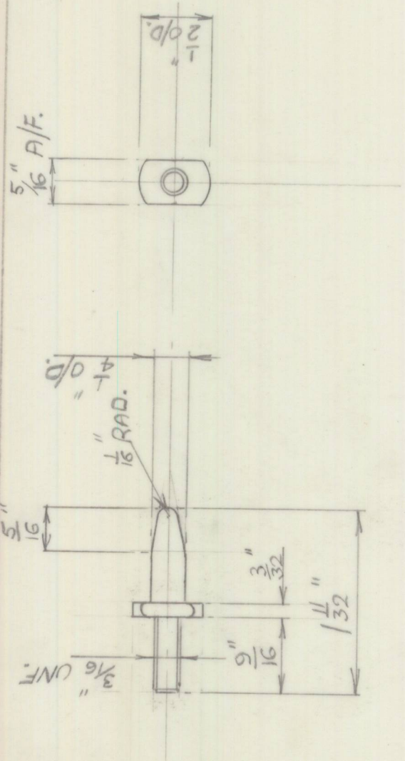
CHASSIS PEG. PB-B-393/2 MAT'L M.S. NICKEL P.
