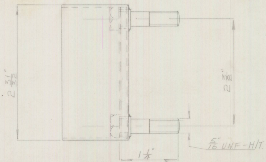
VIEW ON ARROW 'B' ① LOWER MOUNTING BRAKE MASTER CYL.
