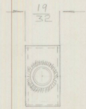
VIEW ON ARROW 'A' ② LOWER MOUNTING CLUTCH MASTER CYL.
