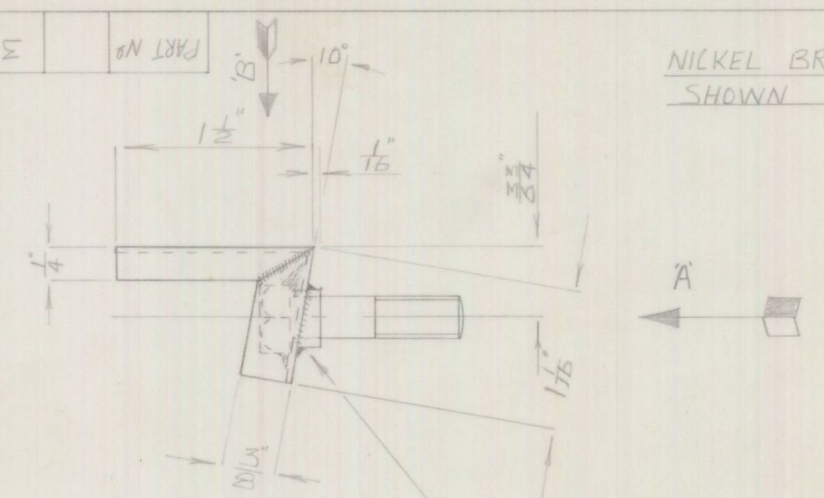
END VIEW OF MOUNTINGS ① & ②
